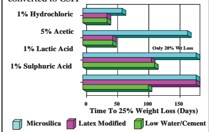
Figure 1 - Acid Resistance. Silica fume chemical resistance concrete is impermeable and \text{Ca}(\text{OH})_2 that is attacked most strongly by acid is converted to CSH
